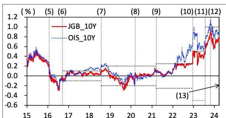
Figure 6: JGB and OIS Rates
