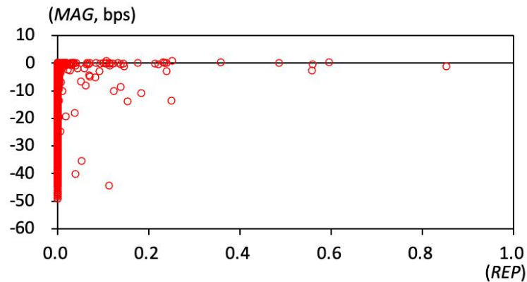
Figure 7: BOJ's JGB Purchase Responses
