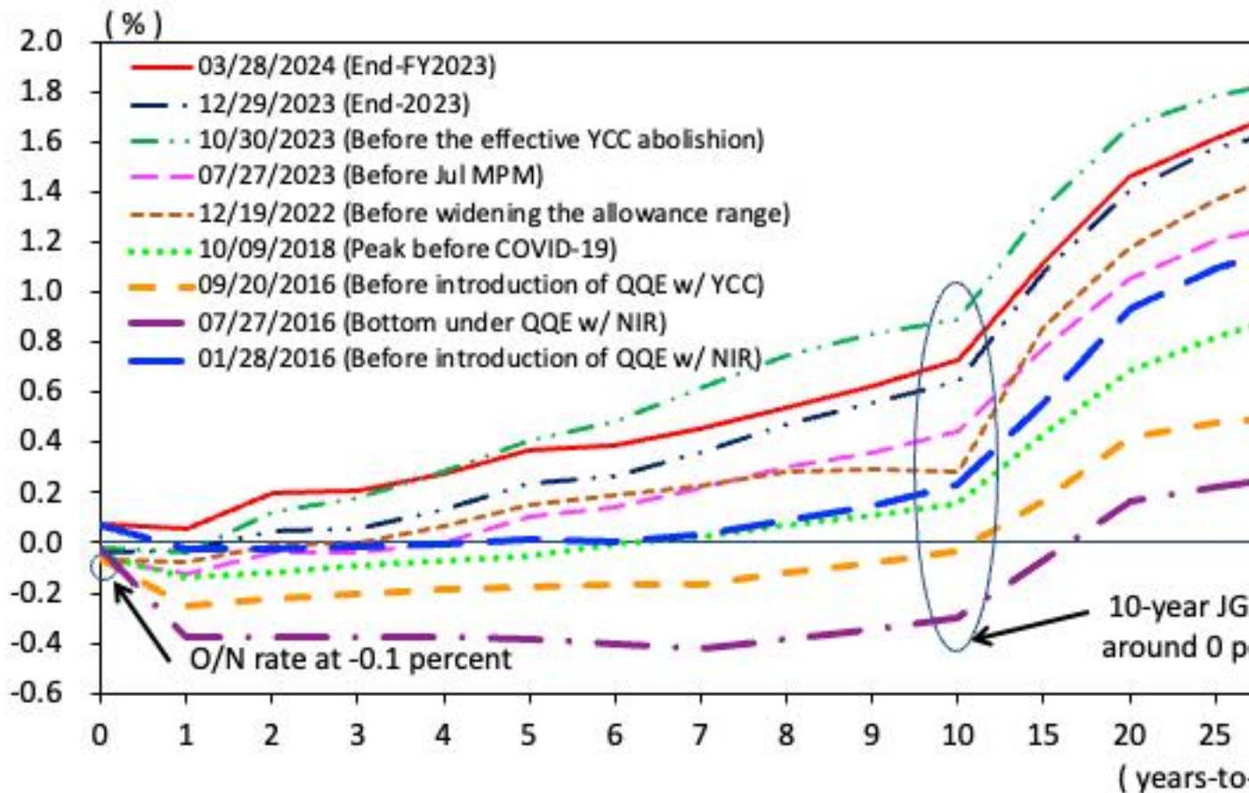
Figure 4: JGB Yield Curve Developments
