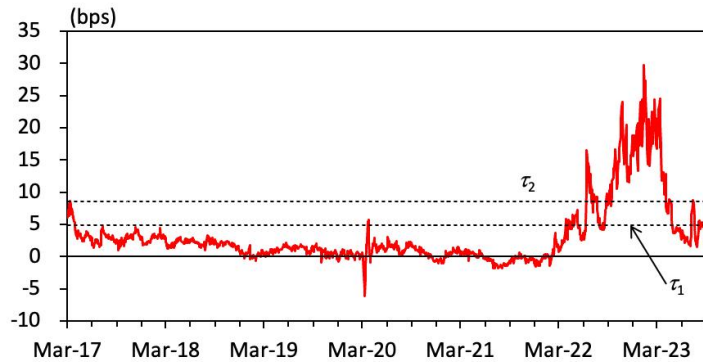
Figure 20: Estimated Threshold Values
