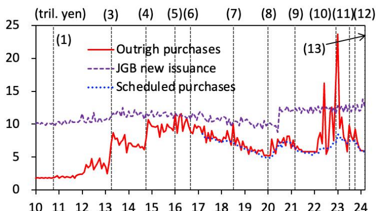
Figure 5: BOJ's JGB Purchases
