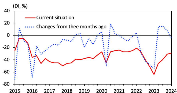
Figure 3: Assessment of JGB Market Functioning
