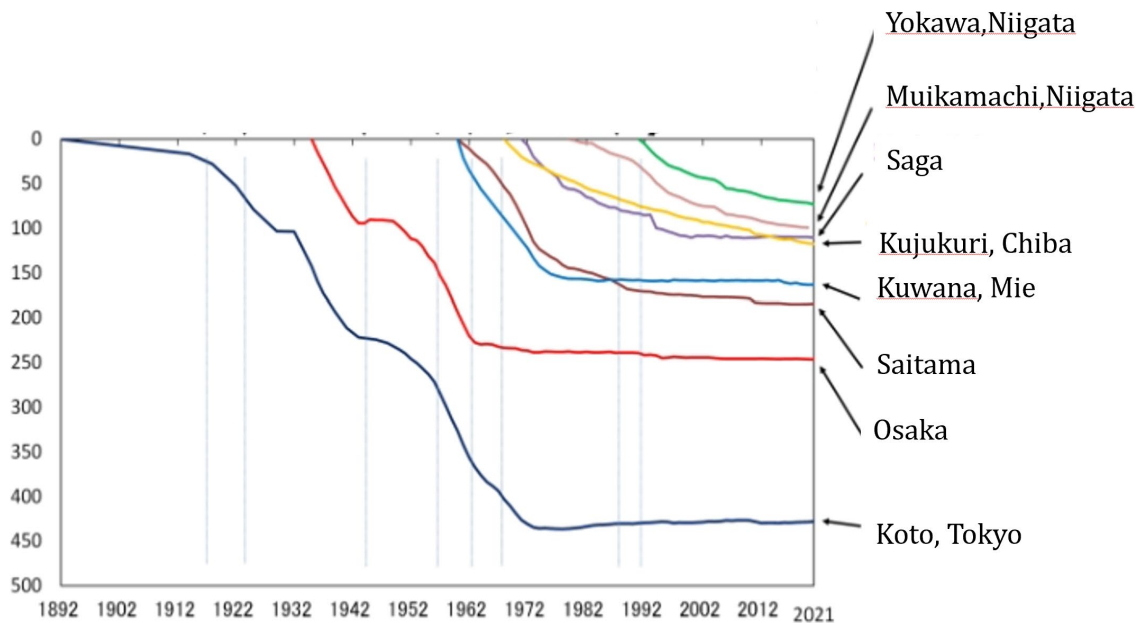
Figure 9. Land subsidence at selected locations in Japan (vertical axis: cumulative subsidence, cm). Source: Ministry of Land, Infrastructure, Transport and Tourism (MLIT), Japan, “Current status of groundwater conservation and land subsidence.” Source: https://www.mlit.go.jp/mizukokudo/mizsei/mizukokudo_mizsei_tk1_000063.html
